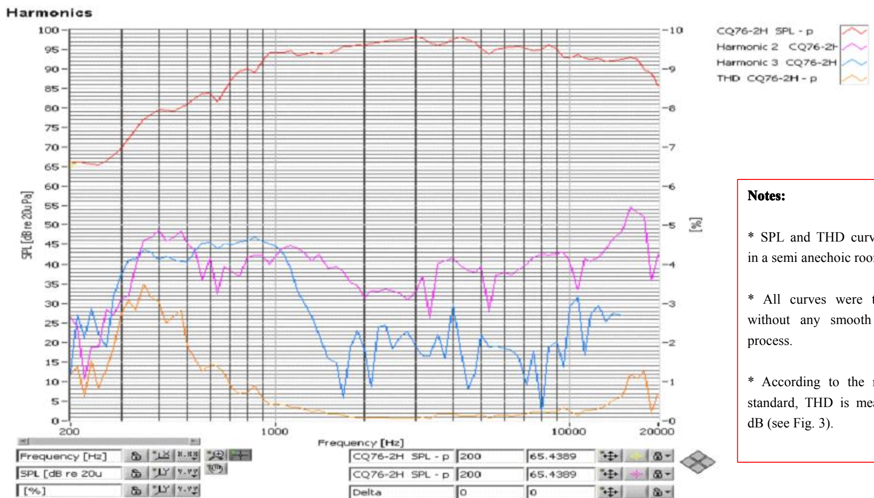
Fig. 3 CQ76-2H THD and 2x,3x harmonics from SoundCheck
