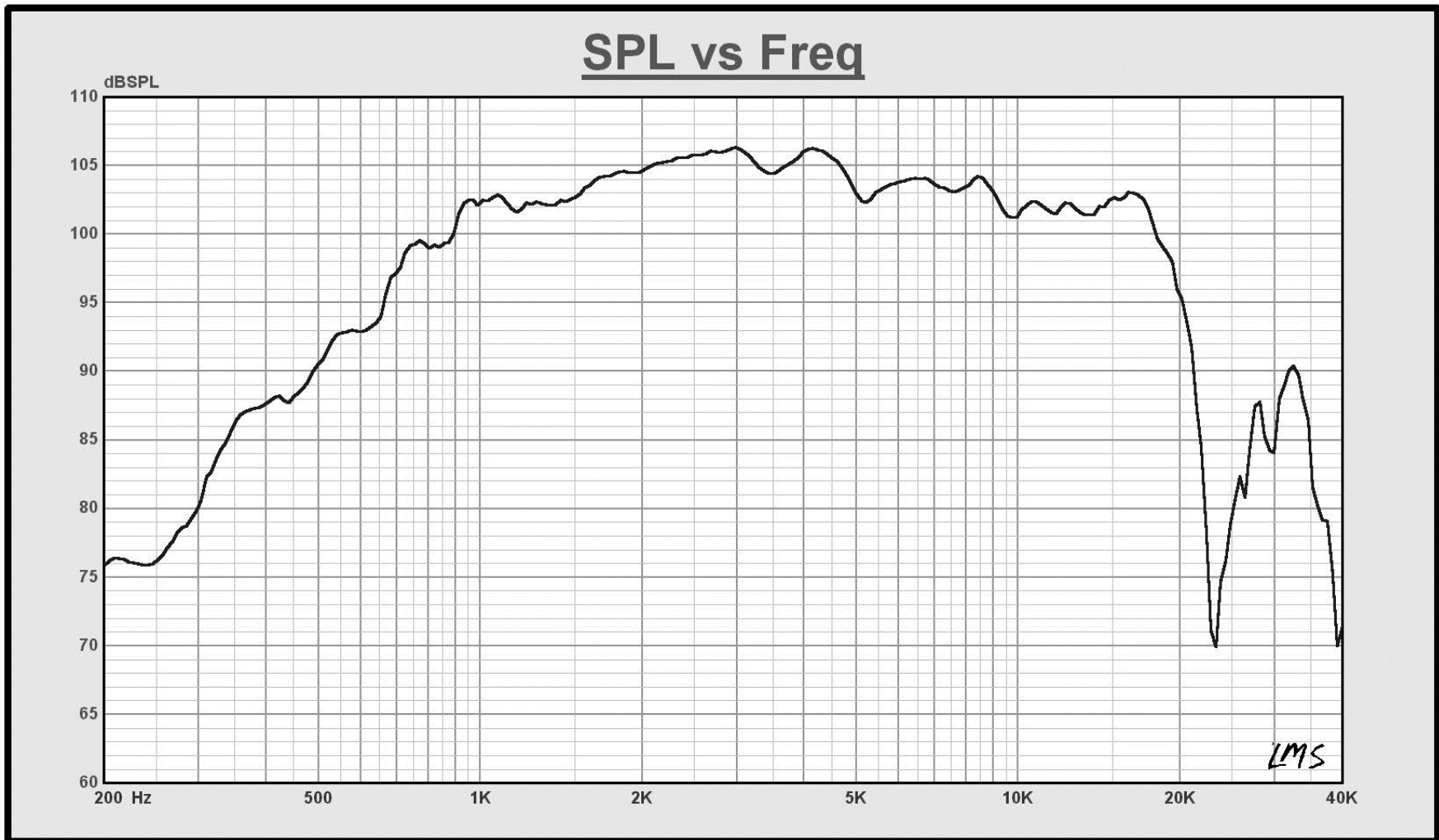
Fig. 1 CQ76-2H SPL curve from LMS
