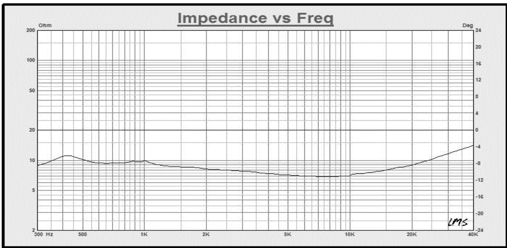
Fig. 2 CQ76-2H Impedance curve from LMS
