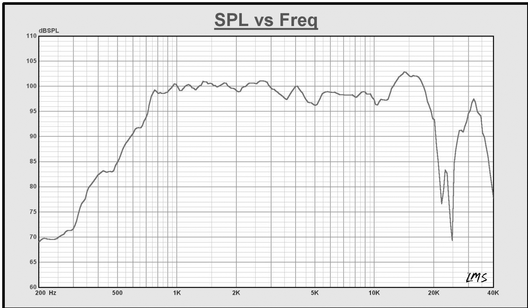
Fig. 1 CQ76-H SPL curve from LMS
