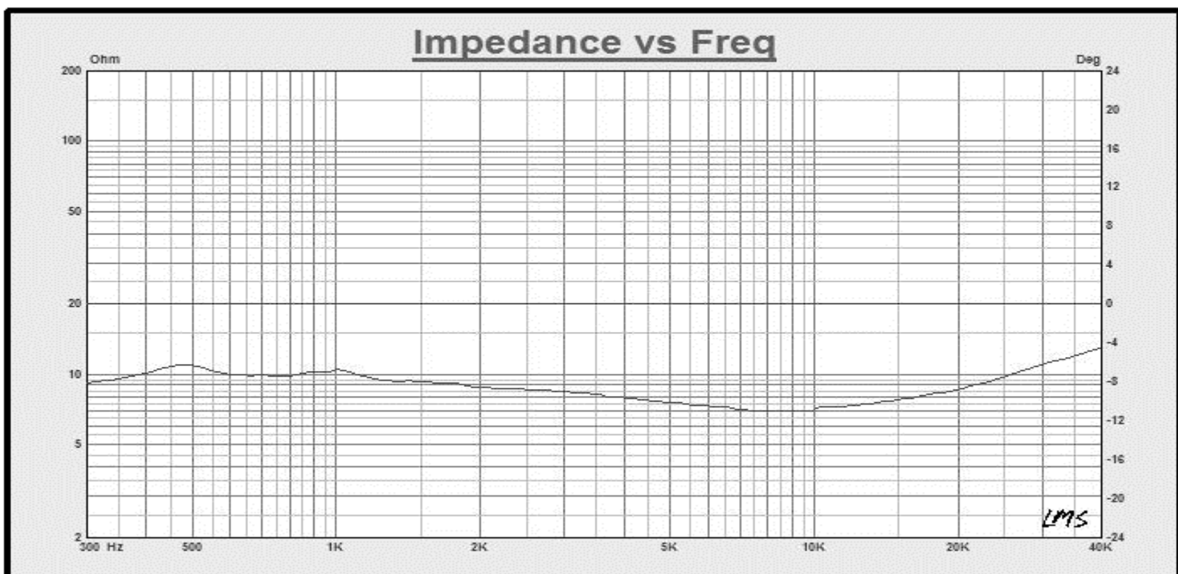
Fig. 2 CQ76-H Impedance curve from LMS
