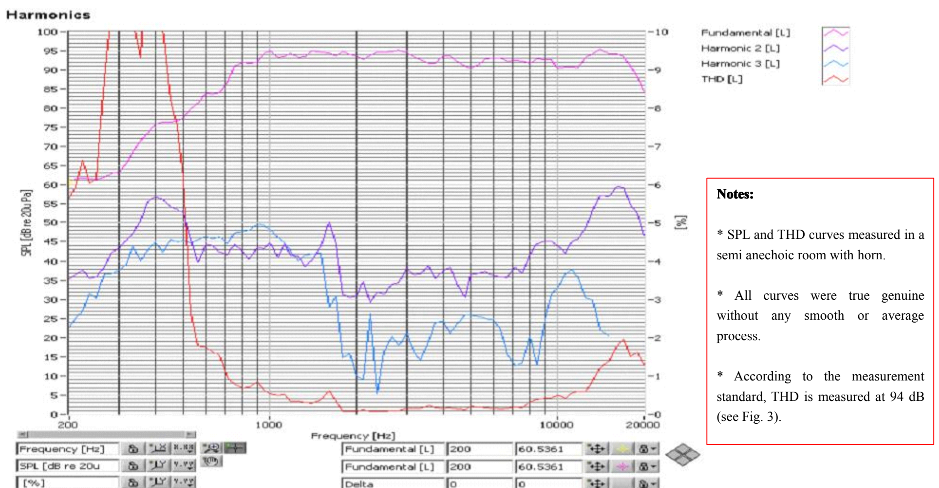
Fig. 3 CQ76-H THD and 2x,3x harmonics from SoundCheck
