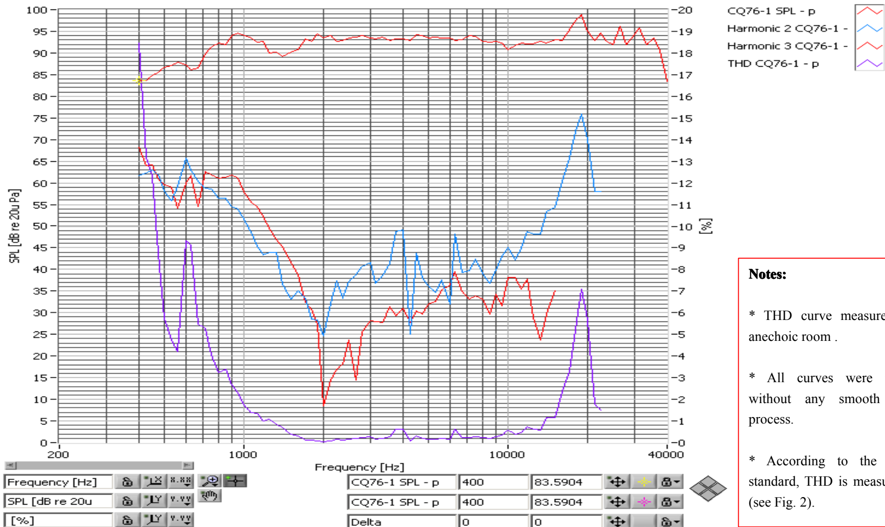
Fig. 2 CQ76 THD and 2x,3x harmonics from SoundCheck
