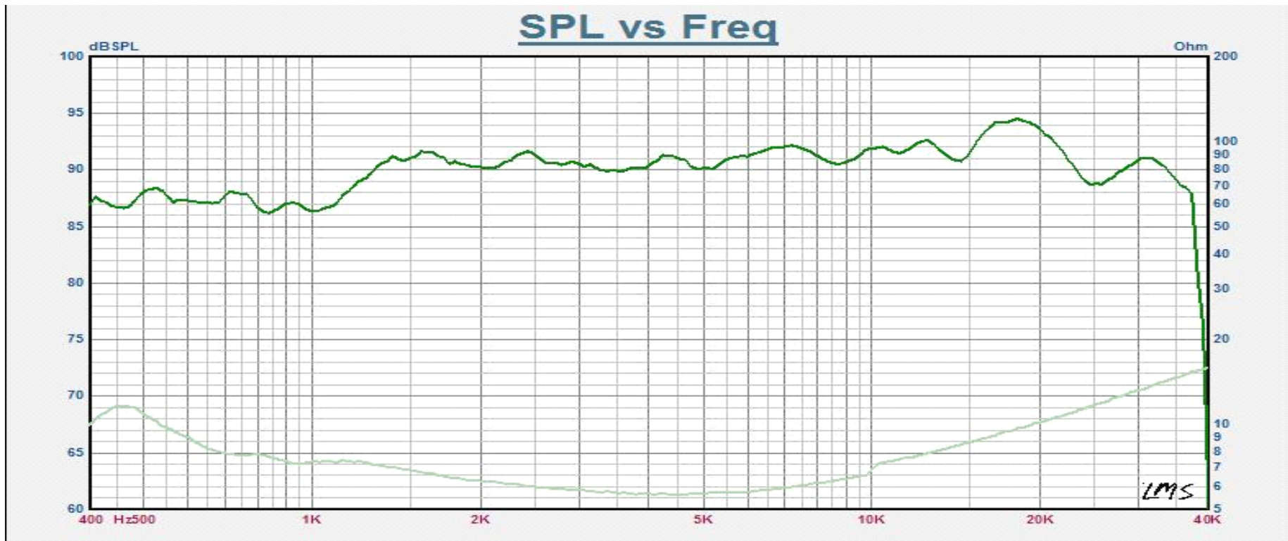
Fig. 1 CQ76 SPL and impedance curves from LMS
