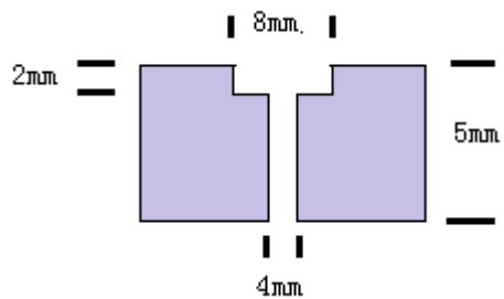
Fig. countersink detailed view(enlarged for readability, the scale is not 1:1, the annotation is correct)
